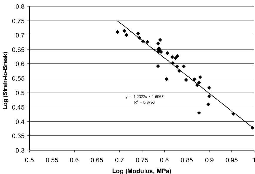
FIG. 10. — Ahagon plot of oven aged tire.
